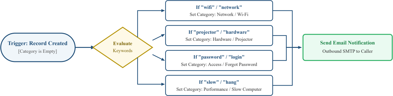
Figure 2: Flow Designer keyword-driven execution logic flowchart.
